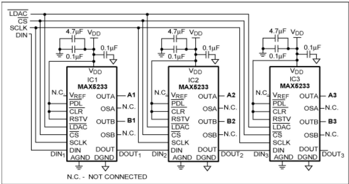
Figure 3. Daisy-chain circuit #1.
