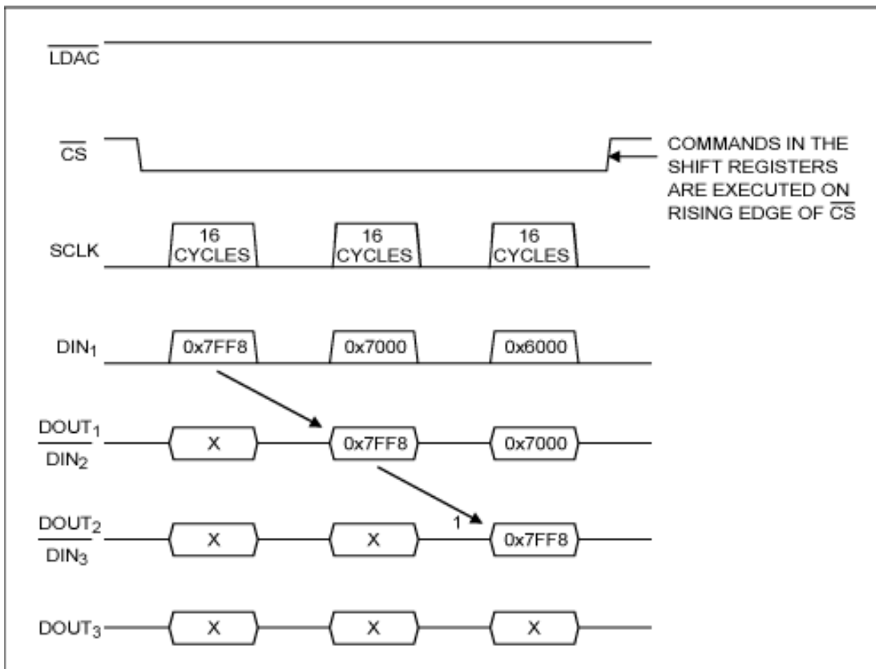
Figure 4. Circuit #1—Command Sequence A.
