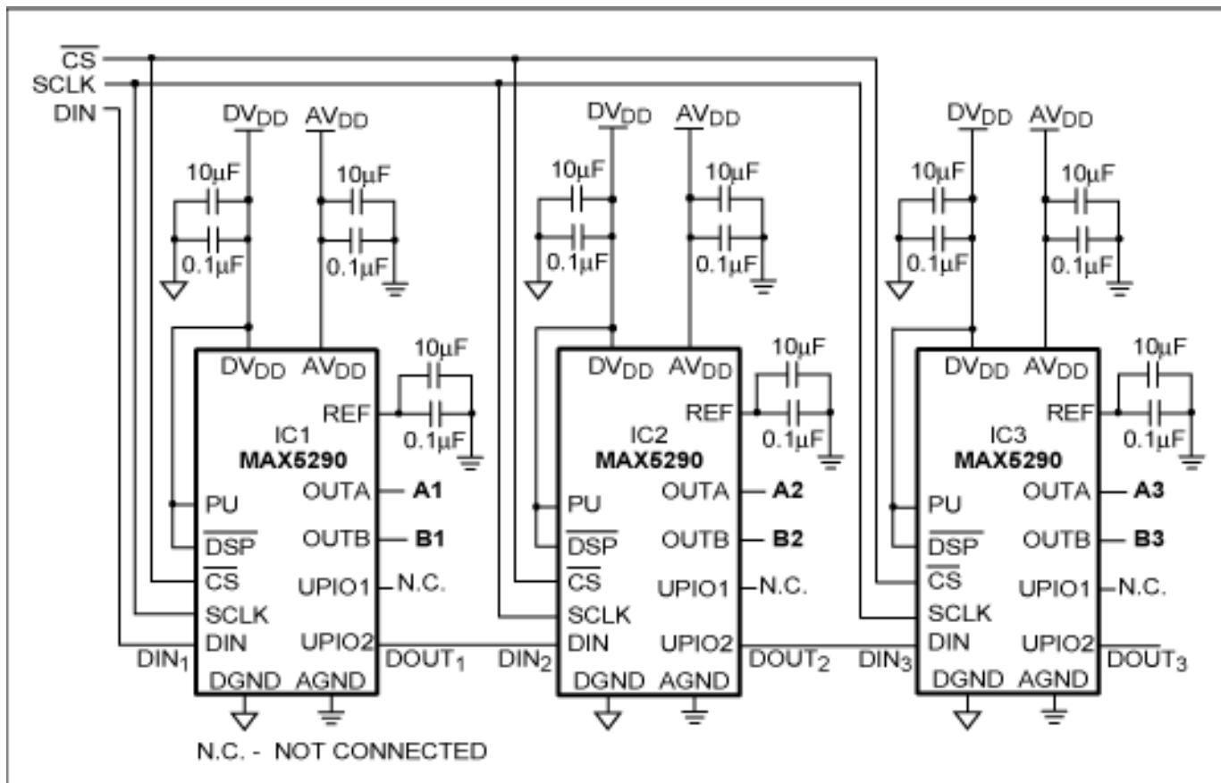
Figure 6. Daisy-chain circuit #2.
