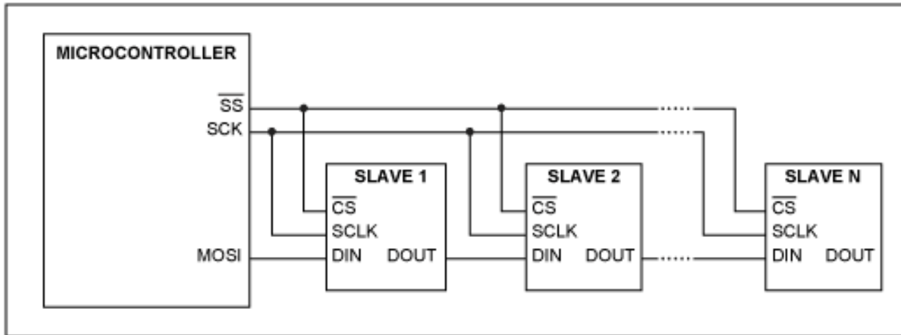
Figure 2. Microcontroller with multiple daisy-chained slave devices.
