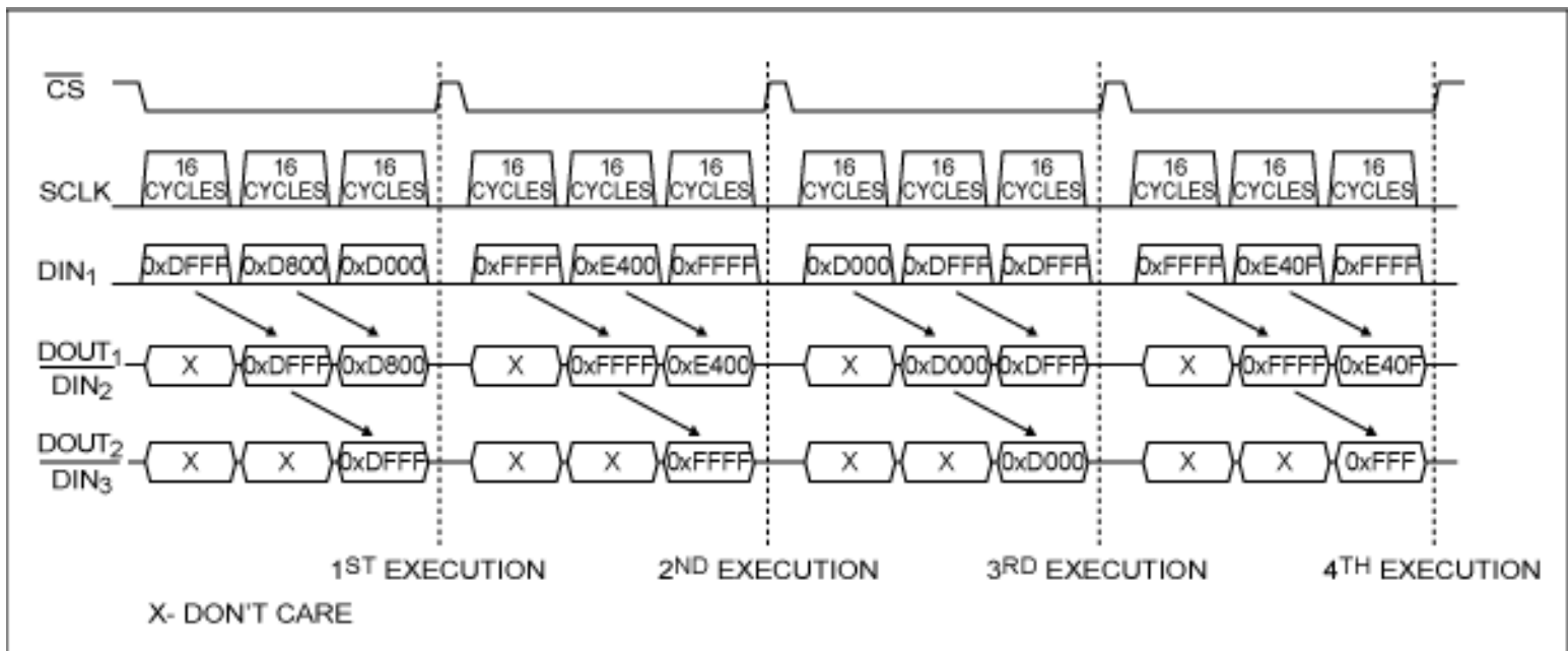
Figure 7. Circuit #2 example command sequence.
