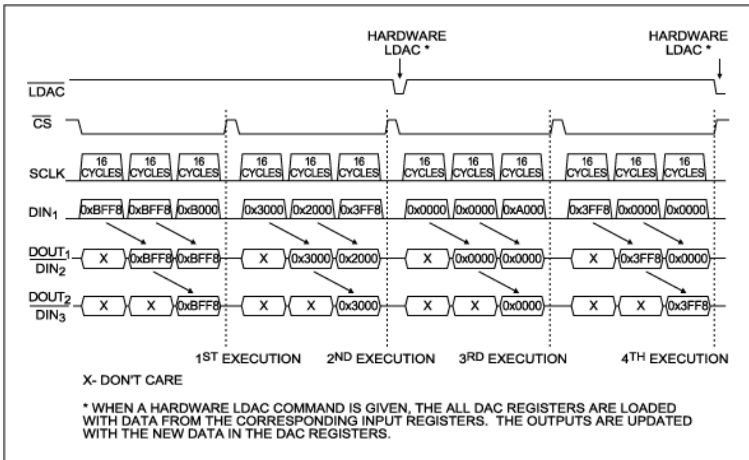
Figure 5. Circuit #1—Command Sequence B.
