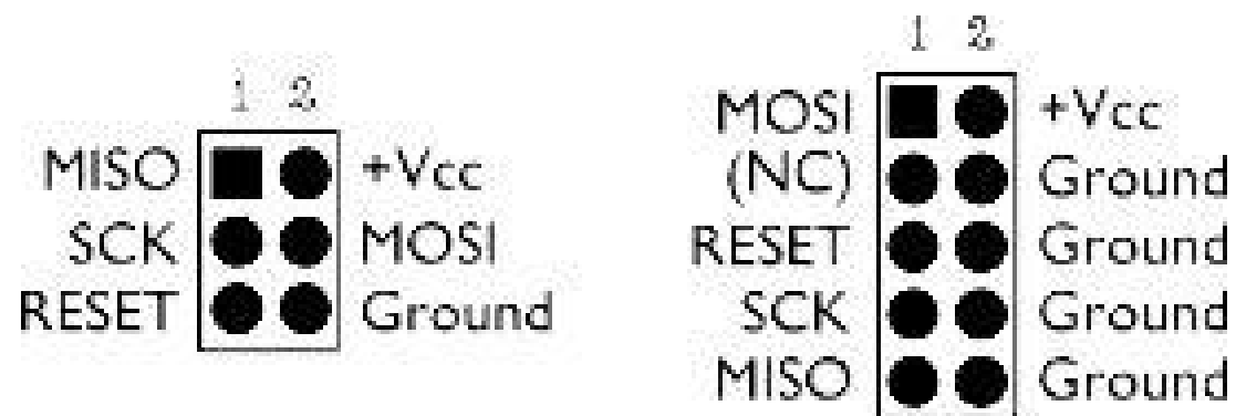
ISP Connectors: 6-pin & 10-pin
