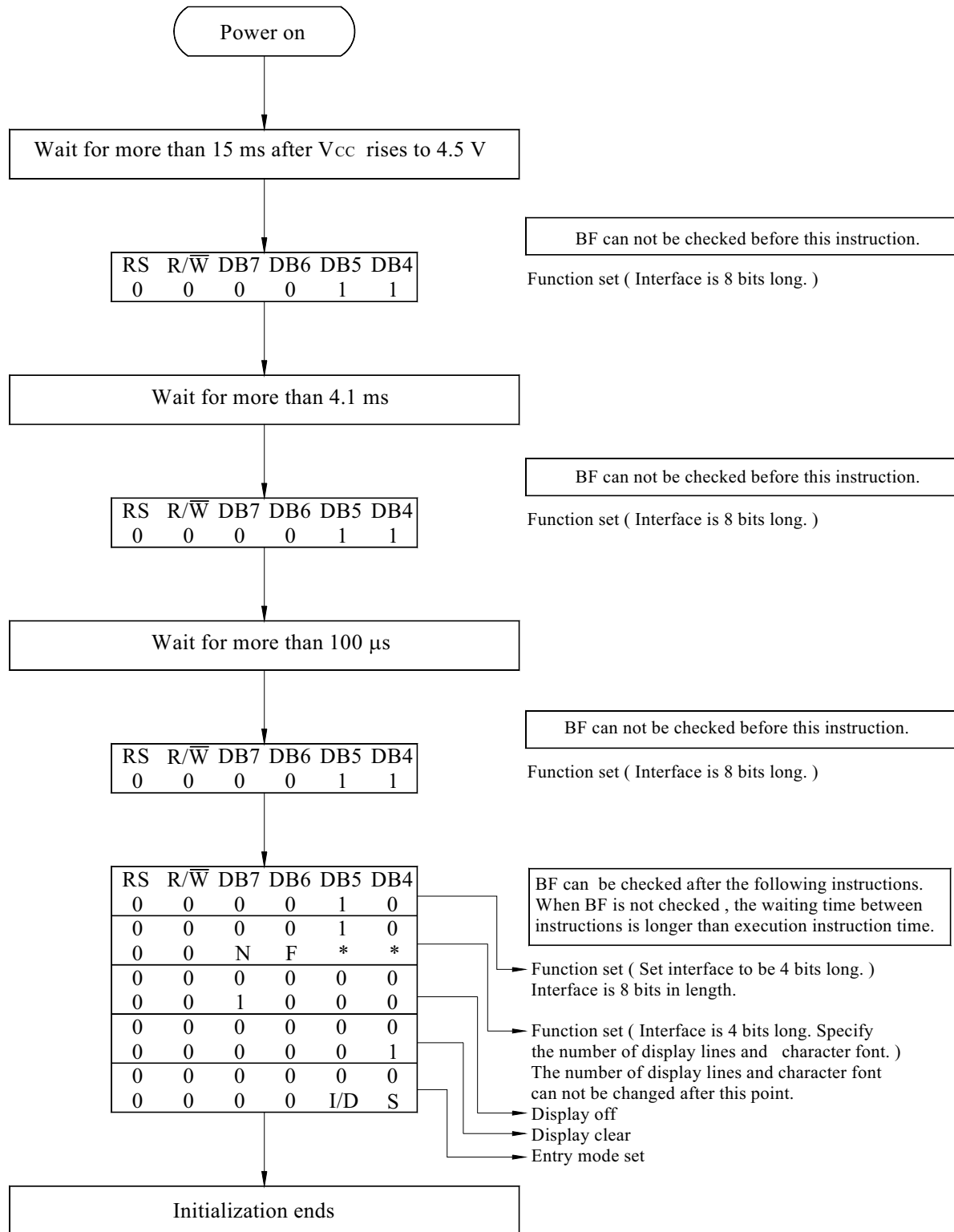
4-Bit Ineterface
