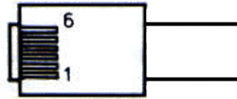
Plug End RJ-11 6 Conductor
