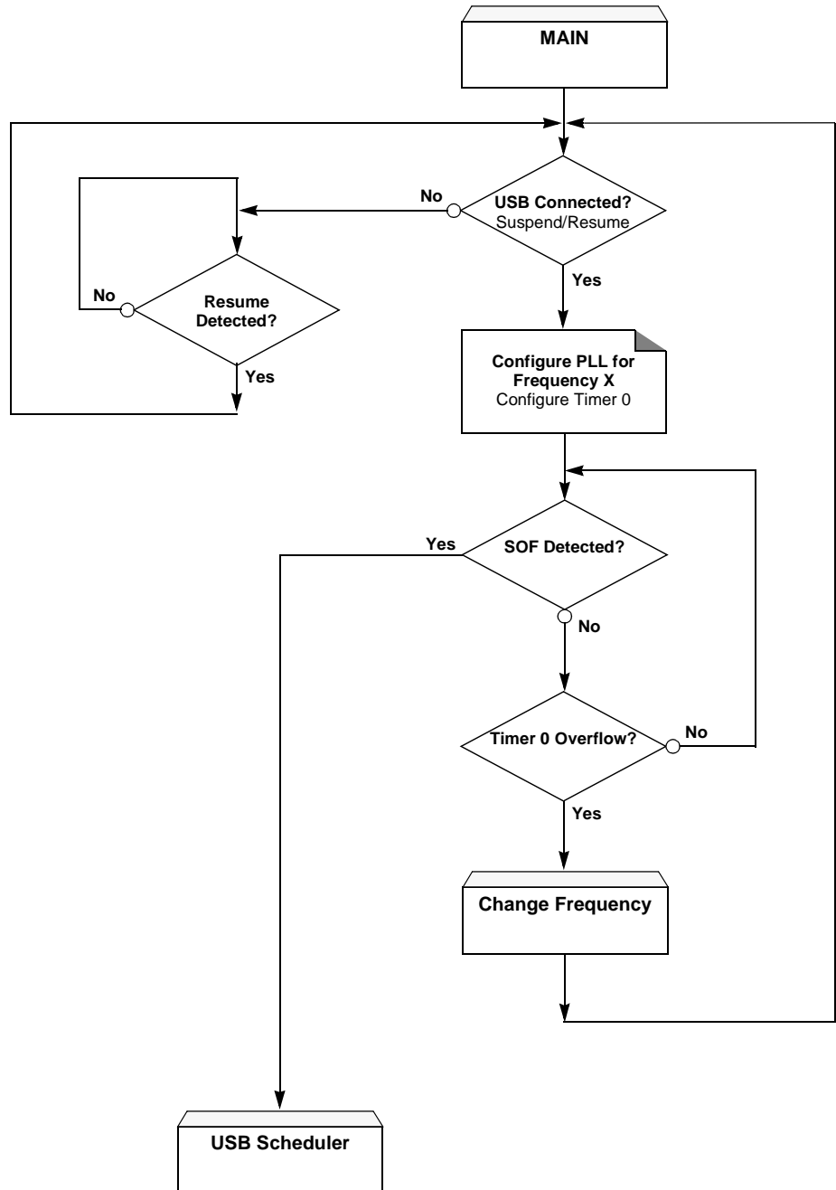
Figure 5. 48 MHz Frequency Auto-generation
